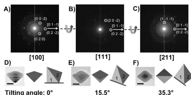
Figure 8. A–C) Tilted SAED pattern of a single bipyramid at different incident angles between the electron beam and the crystal by tilting along the [01-1] direction. D–F) Tilted TEM images (scale bar 50 nm) and schematic illustrations of the top view and side view of the bipyramid at different incident angles.
